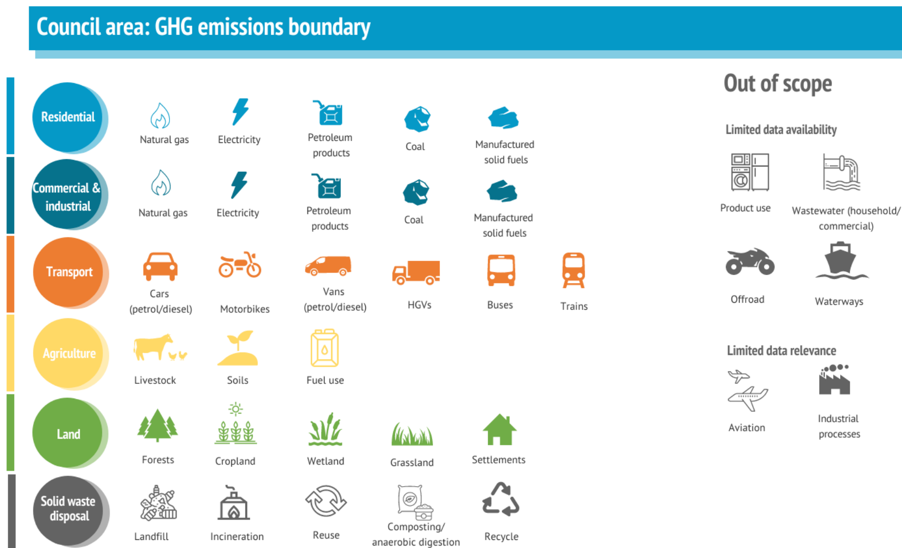
Figure 1: Scope diagram for the borough wide emissions baseline
